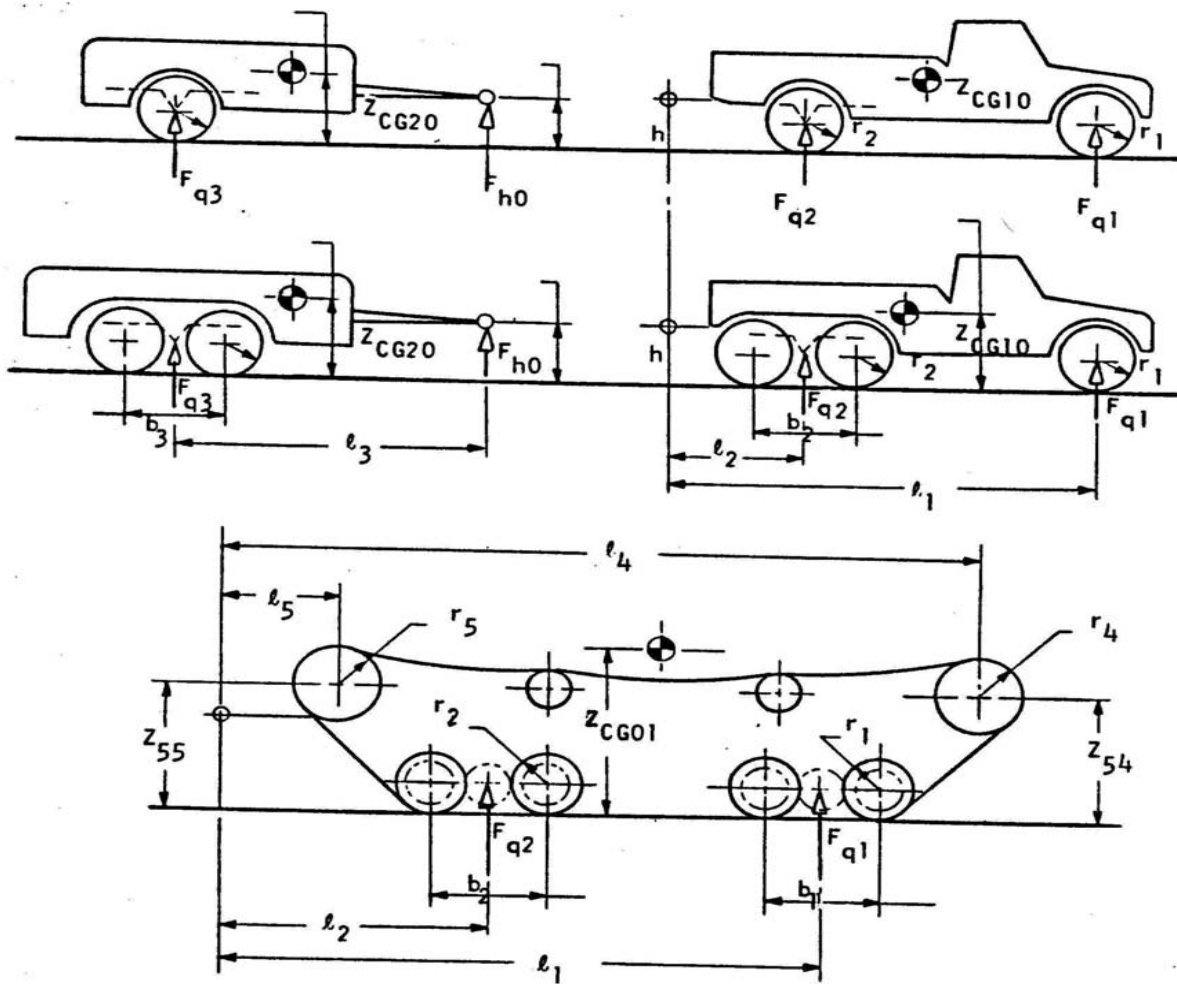
Figure 4-2: Vehicle Configurations [1].
