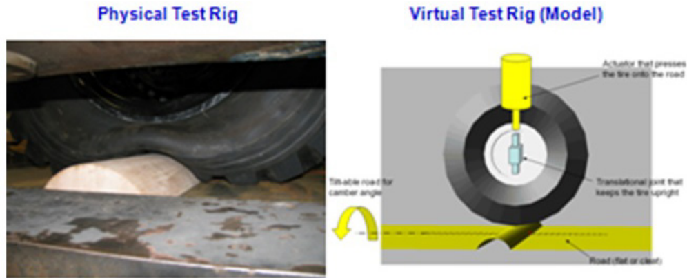
Figure E-12: Correlating Physical Testing with Simulation.
