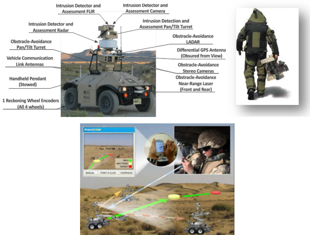
Figure 9-3: Vehicle Intelligence Involves Multiple On-Board Sensors, Autonomy Algorithms, and Interaction with Remote Operators and Resources.
